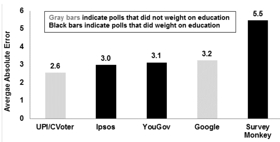
Figure 11. Average Absolute Error on 2016 Presidential margin in Seven Shared Contests, by Five Online Opt-in Polling Organizations. The seven contests for which each of these organizations released estimates in the final two weeks were AZ, FL, GA, NC, OH, PA, and the U.S.
